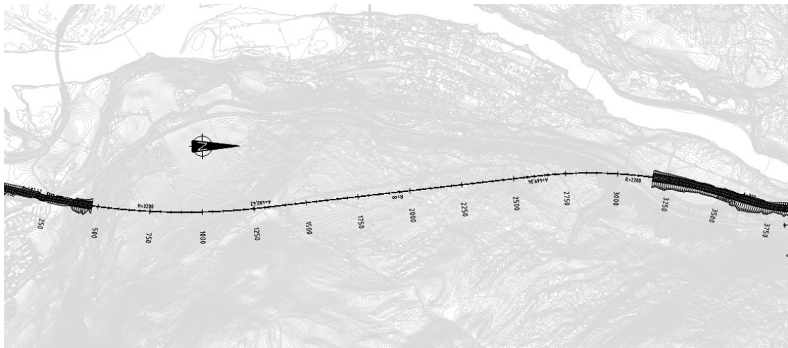
Figur 4-6 Tunnel Storhove – Fåberg
